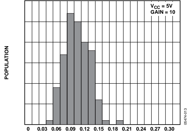
Figure 17. Input Offset Voltage Drift ( \mu\text{V}/^{\circ}\text{C} )
